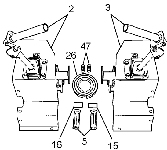
HAND CONTROLS
