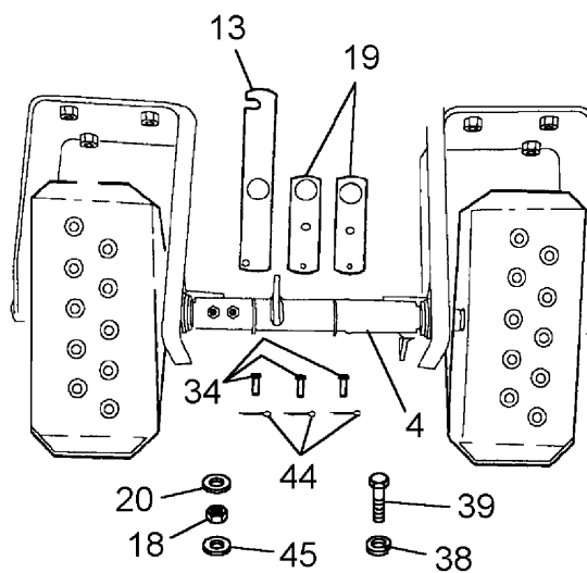
FOOT CONTROLS
