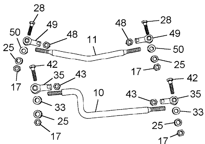
CONTROL RODS
