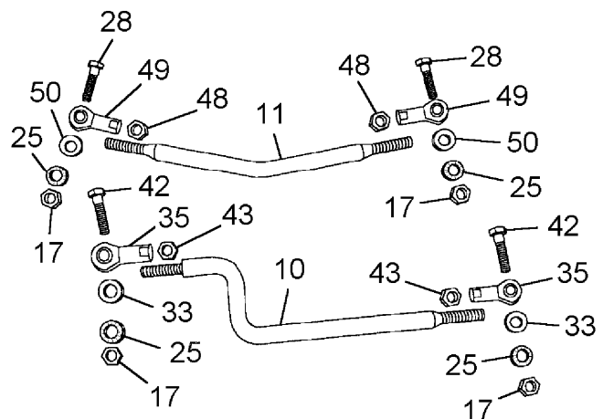
CONTROL RODS
