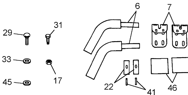
FOREARM RESTS
