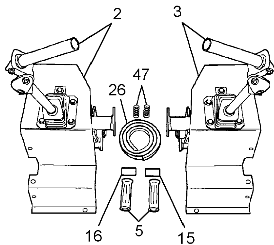
HAND CONTROLS
